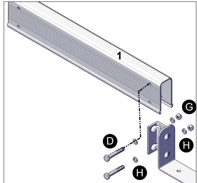
FIGURE 15: FASTEN SHORT U-FRAMES
